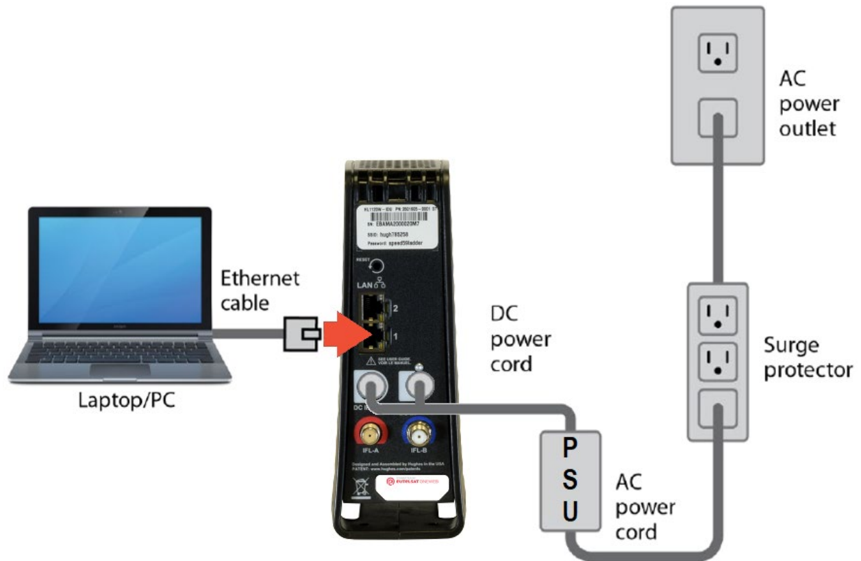
Figure 68: Connecting your laptop to the IDU
