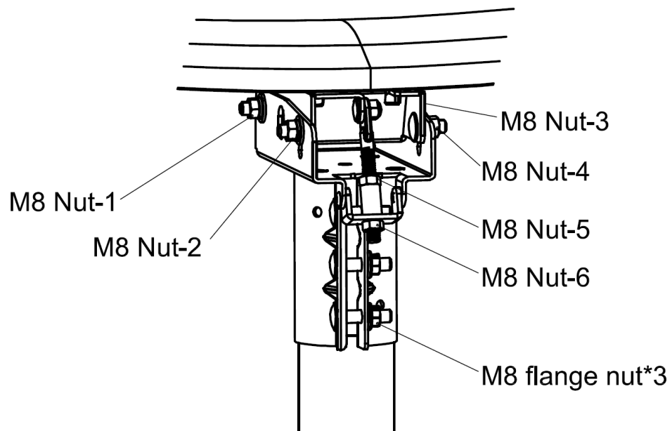
Figure 45: Tightening azimuth and tilt screws
