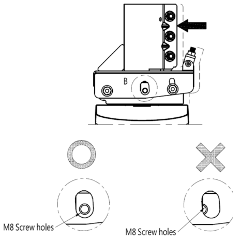
Figure 39: Sliding the mount adapter
