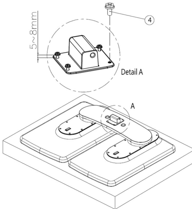
Figure 36: Installing the blind mate guide
