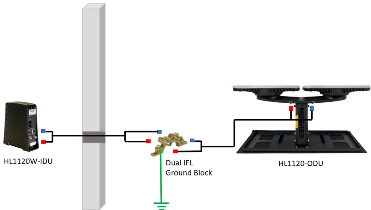
Figure 46: OneWeb HL1120W user terminal – IFL routing
