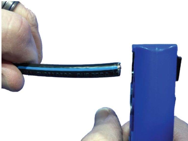
Figure 52: Inserting the IFL cable into the strip tool
