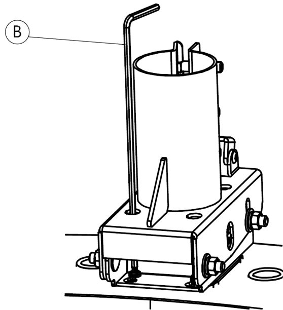
Figure 42: Tightening the blind mate guide screws
