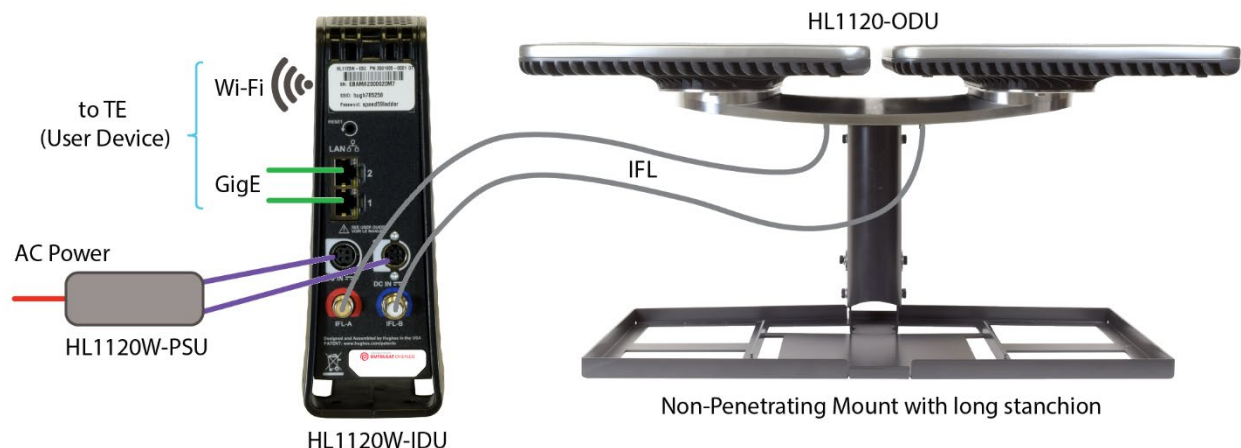
Figure 1: HL1120W satellite user terminal
