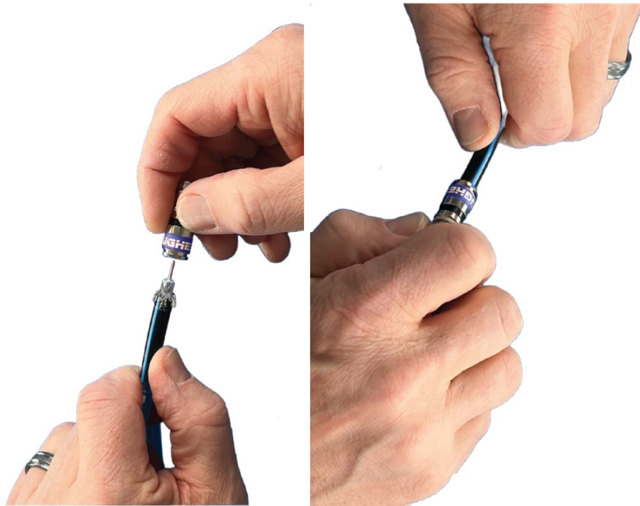
Figure 61: Inserting the IFL cable into the connector
