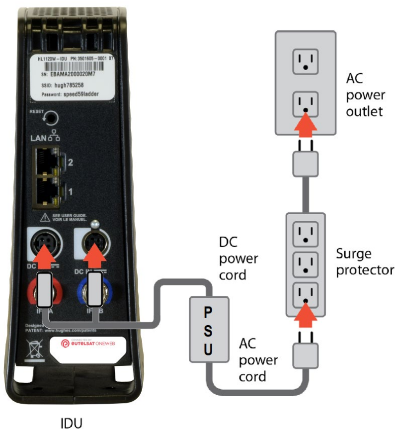
Figure 66: IDU power diagram
