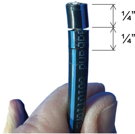
Figure 55: Strip preparation of \frac{1}{4} \times \frac{1}{4} "
