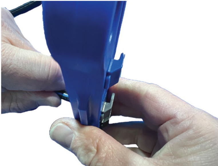
Figure 54: Pulling the cable from the strip tool
