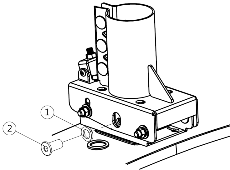
Figure 40: Installing the mount adapter side screws
