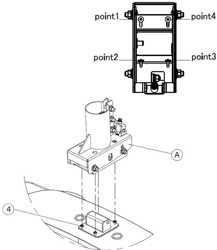
Figure 38: Mounting the mount adapter
